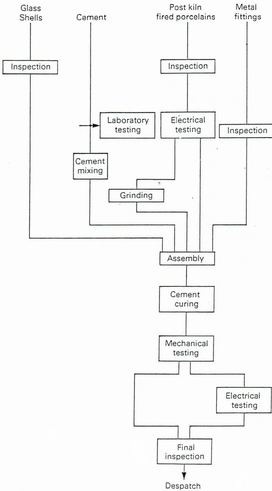
Typical post-kiln processing
